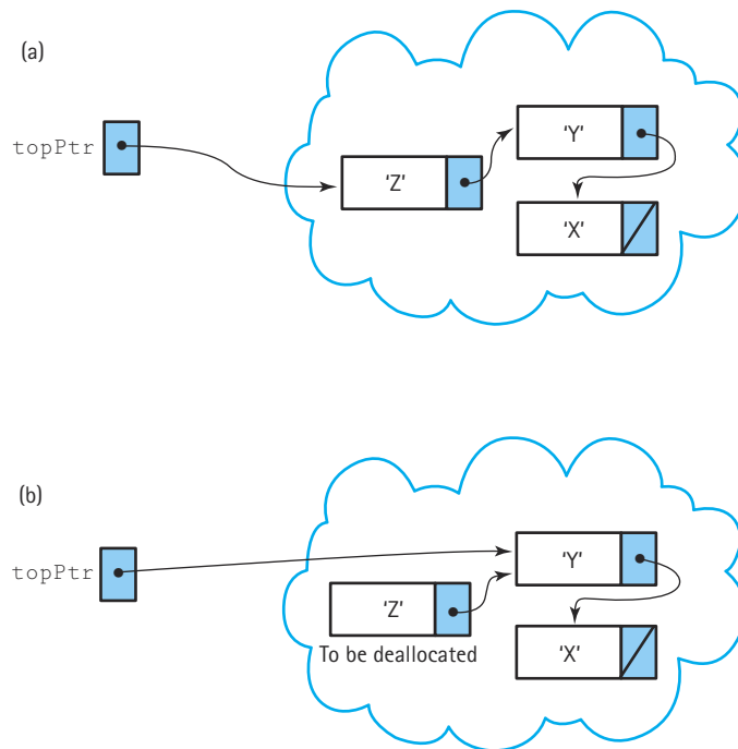
Figure 5.12 Popping the top element
